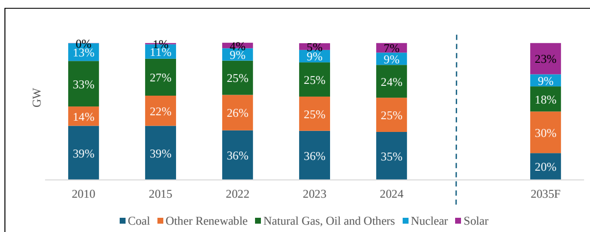
Chart 12: Global Electricity Generation Mix (in %)
