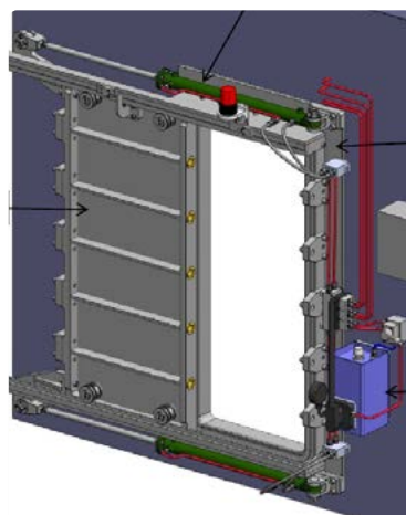
Water Tight Doors indigenised for Coast Guard Vessels
